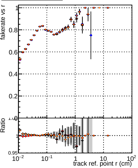
Fake rate vs verpos DOM fit DOM original-0 DOM fit DOM original-127 DOM fit DOM updated-127
