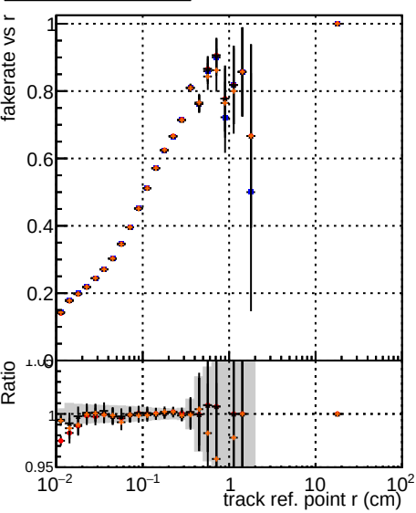
Fake rate vs verpos Legend: DOM, TT, mkFit, DOM original, DOM mod, updated-127
