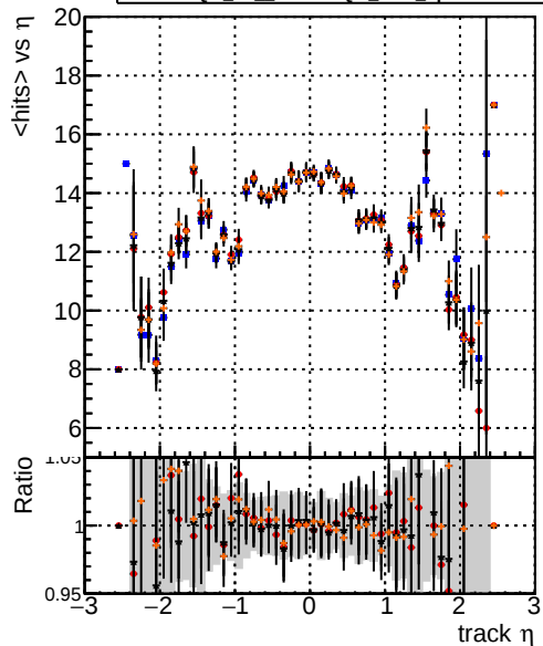
mean hits Legend: DQM_TT mkFit-DQM_original-0 DQM_TT mkFit-DQM_original-127 DQM_TT mkFit-DQM_mod-127 DQM_TT mkFit-DQM_mod_updated-127
