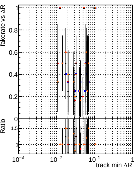
Fake rate vs \Delta R(\text{track, jet}) for various models and updates.
