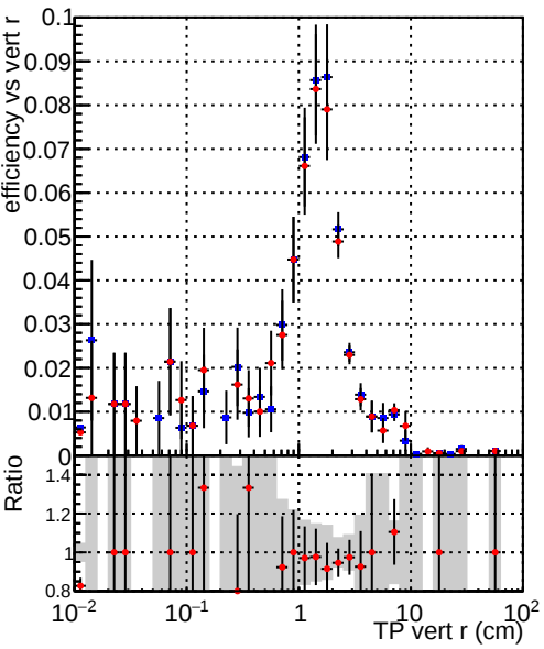
Efficiency vs TP vert r (cm) Legend: DQM_TT_mkFit-DQM_mod-127 (blue points) DQM_TT_mkFit-DQM_mod_updated-127 (red points)
