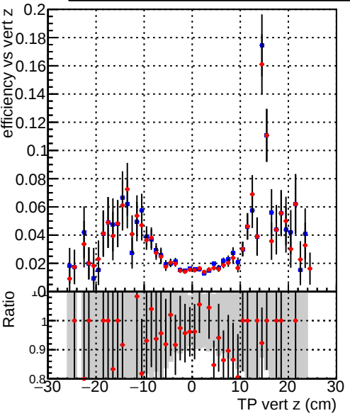
Efficiency vs vertpos Legend: DQM_TT_mkFit-DQM_mod-127 DQM_TT_mkFit-DQM_mod_updated-127
