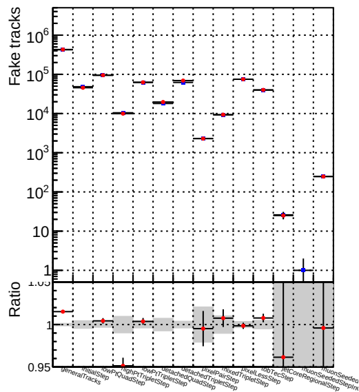
Number —●— DQM_TT__mkFit-DQM_mod_updated-127
