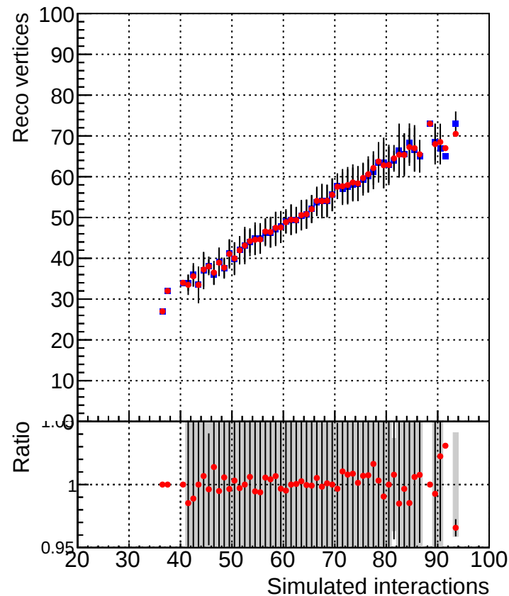
■ DQM_TT_mkFit-DQM_mod-127 ● DQM_TT_mkFit-DQM_mod_updated-127
