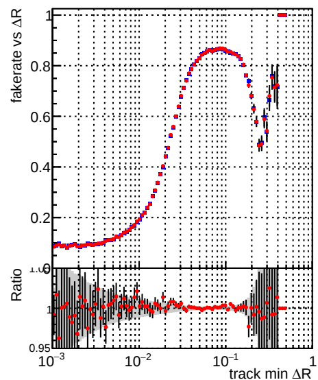
—•— DQM_TT_mkFit-DQM_mod-127 —•— DQM_TT_mkFit-DQM_mod_updated-127
