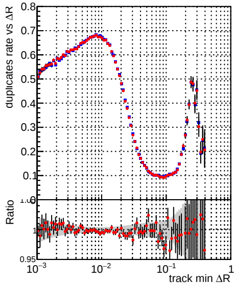
—•— DQM_TT_mkFit-DQM_mod-127 —•— DQM_TT_mkFit-DQM_mod_updated-127
