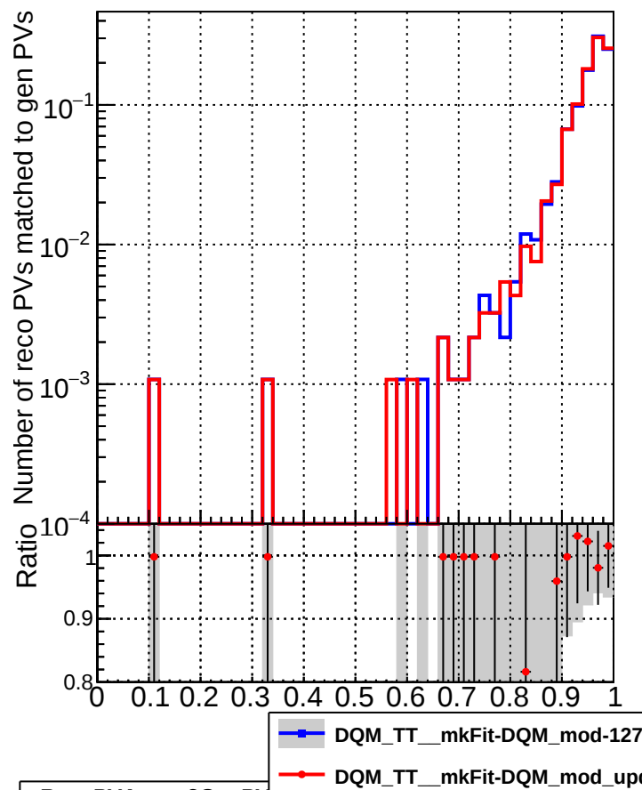
RecoPVAssoc2GenPVMatched_missing
