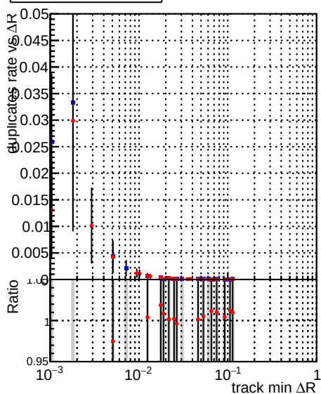
—•— DQM_TT_mkFit-DQM_mod-127 —•— DQM_TT_mkFit-DQM_mod_updated-127
