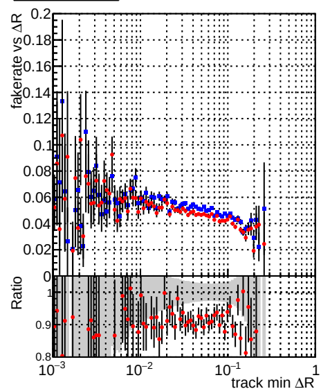
—•— DQM_TT_mkFit-DQM_mod-127 —•— DQM_TT_mkFit-DQM_mod_updated-127
