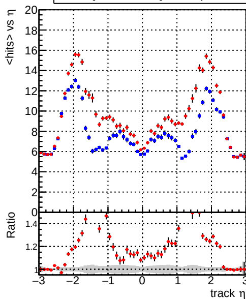
mean hits Legend: DQM_TT_mkFit-DQM_mod-127 (blue line), DQM_TT_mkFit-DQM_mod_updated-127 (red line)
