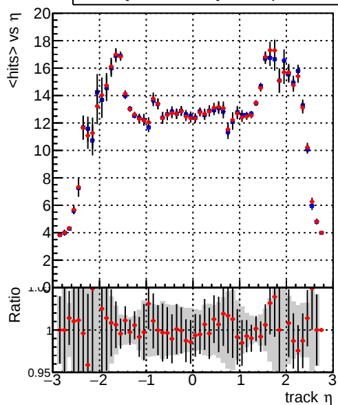
mean hits — DQM_TT_mkFit-DQM_mod-127 — DQM_TT_mkFit-DQM_mod_updated-127
