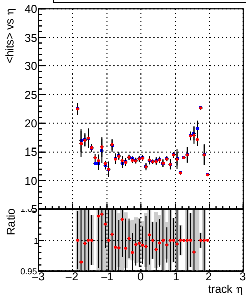
mean hit — DQM_TT_mkFit-DQM_mod-127 — DQM_TT_mkFit-DQM_mod_updated-127
