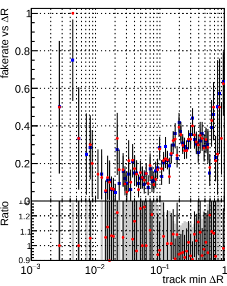
Fake rate vs \Delta R(\text{track, jet}) Legend: DQM_TT_mkFit-DQM_mod-127 (blue diamonds), DQM_TT_mkFit-DQM_mod_updated-127 (red circles)
