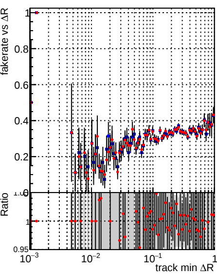
Legend: DQM_TT_mkFit-DQM_mod-127 (blue line with markers), DQM_TT_mkFit-DQM_mod_updated-127 (red line with markers)
