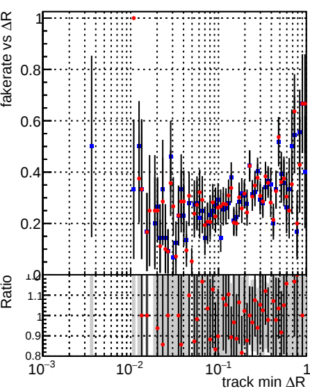
Fake rate vs \Delta R(\text{track, jet}) Legend: DQM_TT_mkFit-DQM_mod-127 (blue stars), DQM_TT_mkFit-DQM_mod_updated-127 (red stars)
