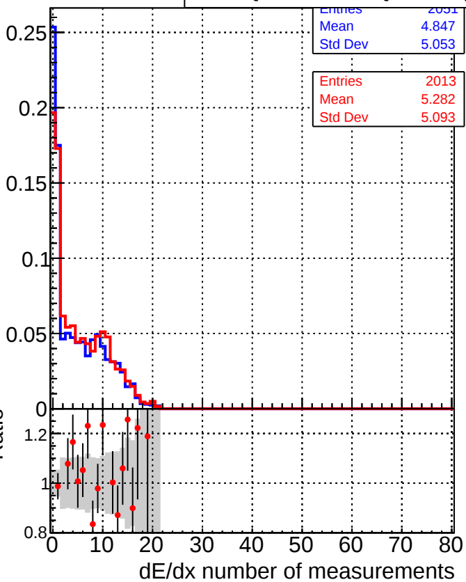
—■— DQM_TT_mkFit-DQM_mod-127 —●— DQM_TT_mkFit-DQM_mod_updated-127
