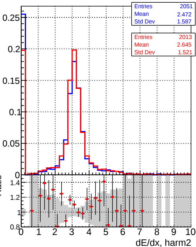
—■— DQM_TT_mkFit-DQM_mod-127 —●— DQM_TT_mkFit-DQM_mod_updated-127
