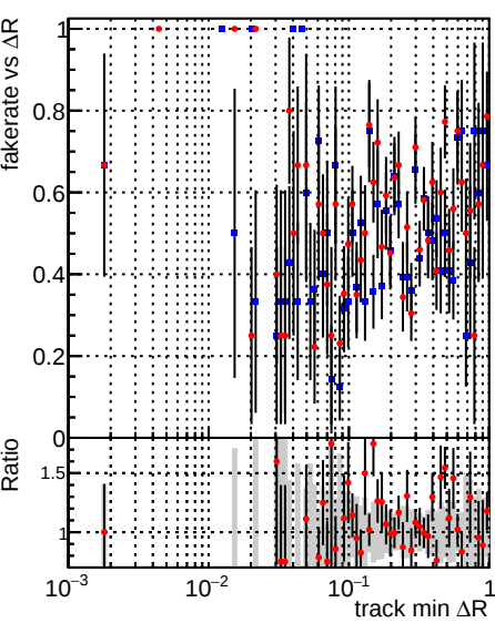
Fake rate vs \Delta R(\text{track, jet}) Legend: DQM_TT_mkFit-DQM_mod-127 (blue squares), DQM_TT_mkFit-DQM_mod_updated-127 (red circles)
