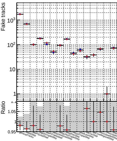
Number —●— DQM_TT_mkFit-DQM_mod_updated-127
