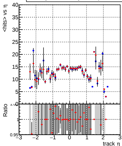
mean hit Legend: — DQM_TT_mkFit-DQM_mod-127 — DQM_TT_mkFit-DQM_mod-updated-127
