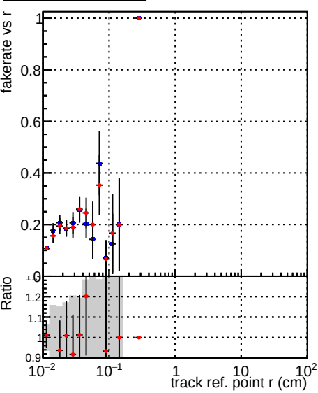
■ DQM_TT_mkFit-DQM_mod-127 ● DQM_TT_mkFit-DQM_mod_updated-127
