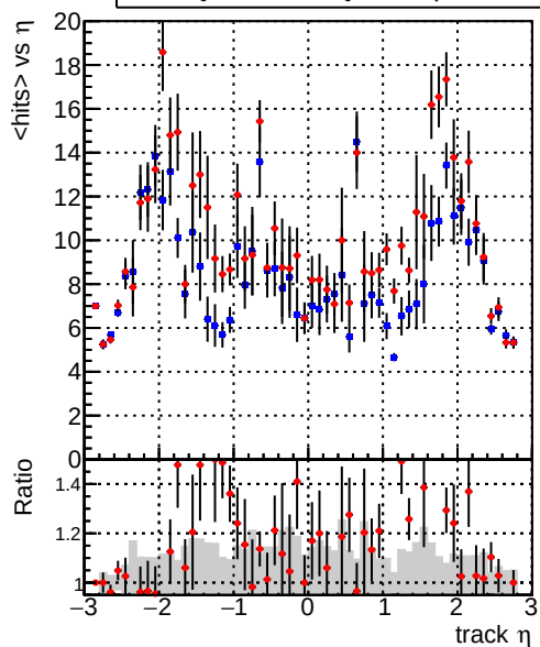
mean hit — DQM_TT_mkFit-DQM_mod-127 — DQM_TT_mkFit-DQM_mod-127
