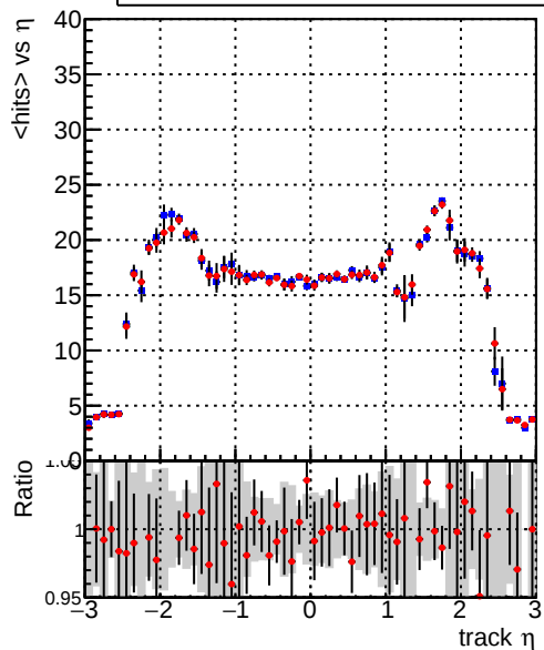
mean hit Legend: DQM_TT_mkFit-DQM_mod-127 (blue line with circles), DQM_TT_mkFit-DQM_mod_updated-127 (red line with circles)
