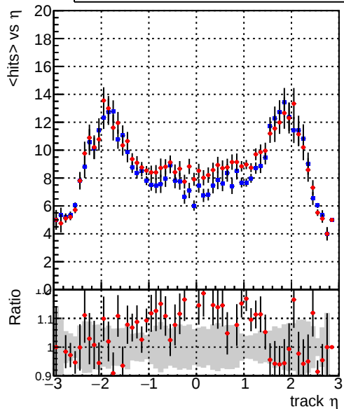
mean hit — DQM_TT_mkFit-DQM_mod-127 — DQM_TT_mkFit-DQM_mod_updated-127
