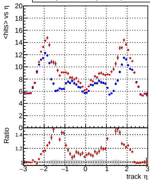
mean hits vs \eta Legend: DQM_TT_mkFit-DQM_mod-127 (blue line), DQM_TT_mkFit-DQM_mod_updated-127 (red line)
