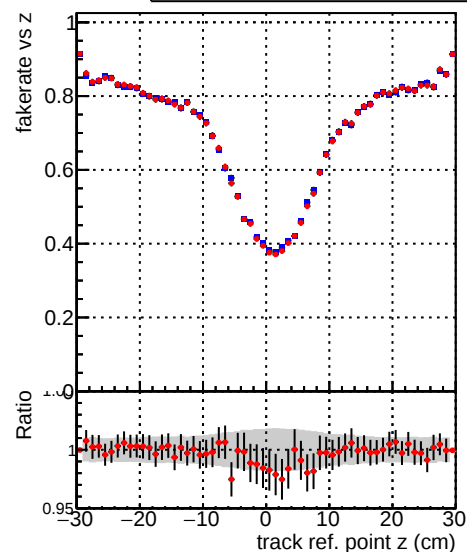
—●— DQM_TT_mkFit-DQM_mod-127 —●— DQM_TT_mkFit-DQM_mod_updated-127
