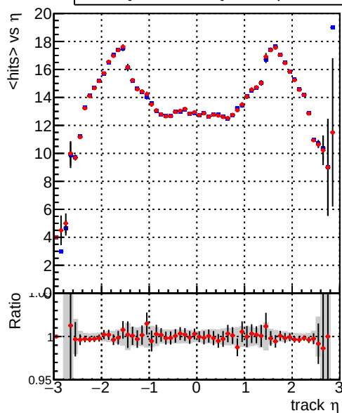
— DQM_TT_mkFit-DQM_mod-127 — DQM_TT_mkFit-DQM_mod_updated-127 mean hits vs \eta
