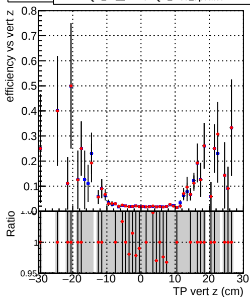
Efficiency vs vert z —●— DQM_TT_mkFit-DQM_mod-127 —●— DQM_TT_mkFit-DQM_mod_updated-127
