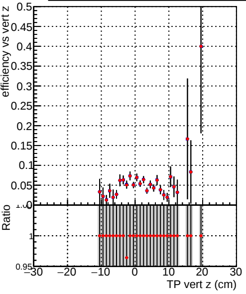
Efficiency vs vert z Legend: DQM_TT_mkFit-DQM_mod-127 DQM_TT_mkFit-DQM_mod_updated-127
