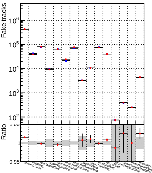
Number —●— DQM_TT_mkFit-DQM_mod_updated-127
