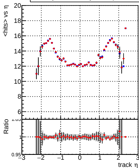
mean hits vs \eta — DQM_TT_mkFit-DQM_mod-127 — DQM_TT_mkFit-DQM_mod_updated-127
