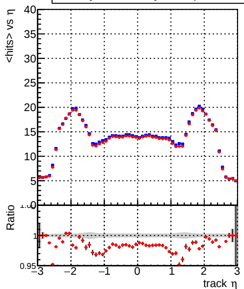
— DQM_TT_mkFit-DQM_mod-127 — DQM_TT_mkFit-DQM_mod_updated-127 mean hits
