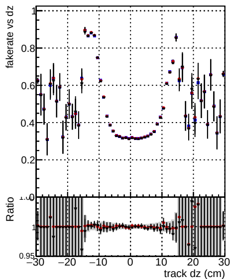
Fake rate vs dz DOM TT mkFit-DOM original-0 DOM TT mkFit-DOM mod updated-127
