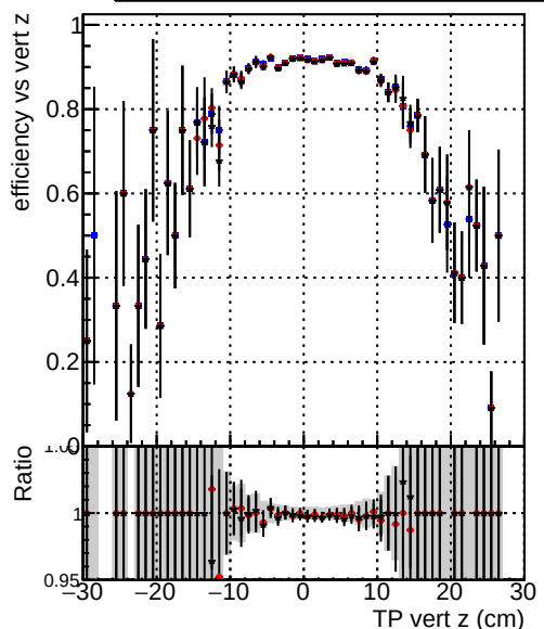
Efficiency vs. TP vert z — DQM_TT_mkFit-DQM_original-0 — DQM_TT_mkFit-DQM_mod-127 — DQM_TT_mkFit-DQM_mod_updated-127
