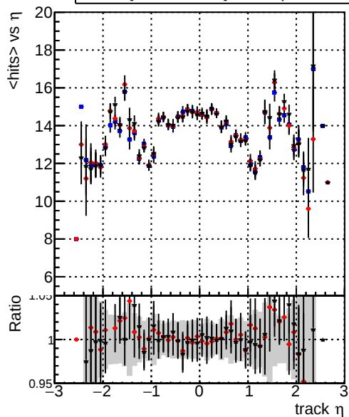
DQM_TT_mkFit-DQM_original-0 DQM_TT_mkFit-DQM_mod-127 DQM_TT_mkFit-DQM_mod_updated-127 mean hits
