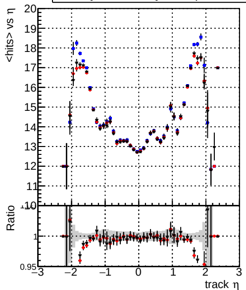
mean hits vs \eta — DQM_TT_mkFit-DQM_original-0 — DQM_TT_mkFit-DQM_mod-127 — DQM_TT_mkFit-DQM_mod_updated-127
