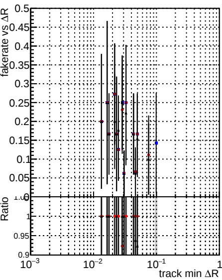
Legend: - \Delta R TT mkFit-DQM original-0 - \Delta R TT mkFit-DQM mod-127 - \Delta R TT mkFit-DQM mod_updated-127
