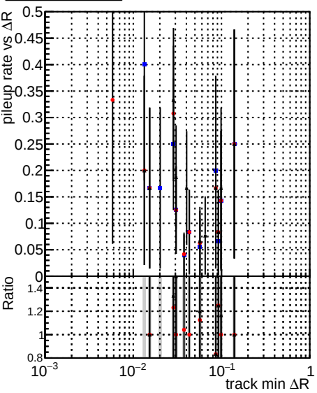
Legend: - \Delta R TT mkFit-DQM original-0 - \Delta R TT mkFit-DQM mod-127 - \Delta R TT mkFit-DQM mod_updated-127
