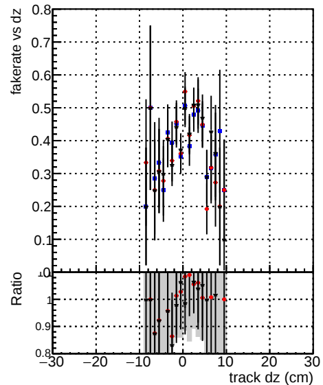
Fake rate vs dz Legend: DOM TT mkFit-DOM-original-0 (blue dots) DOM TT mkFit-DOM-mod-127 (red dots) DOM TT mkFit-DOM-mod-updated-127 (black dots)
