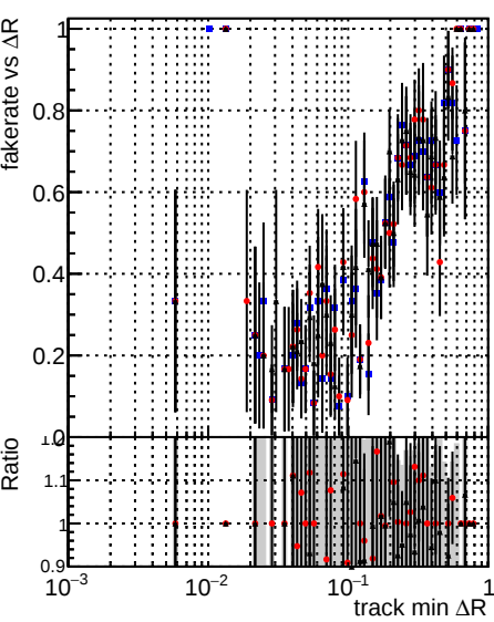
Fake rate vs \Delta R(\text{track, jet}) Legend: DQM TT mkFit-DQM original-0 (blue dots) DQM TT mkFit-DQM mod-127 (red dots) DQM TT mkFit-DQM mod-updated-127 (black dots)
