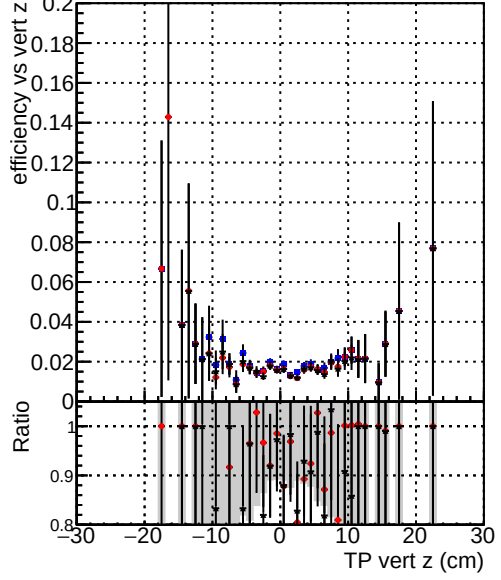
Efficiency vs. sim PV z —●— DQM_TT_mkFit-DQM_original-0 —●— DQM_TT_mkFit-DQM_mod-127 —●— DQM_TT_mkFit-DQM_mod_updated-127
