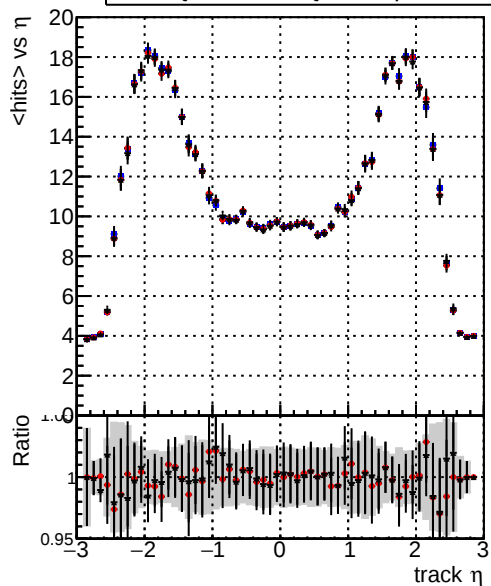
mean hits vs \eta Legend: DQM_TT_mkFit-DQM_original-0 (blue), DQM_TT_mkFit-DQM_mod-127 (red), DQM_TT_mkFit-DQM_mod_updated-127 (black)
