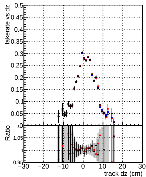
Fake rate vs dz Legend: DOM TT mkFit-DOM original-0 DOM TT mkFit-DOM mod updated-127
