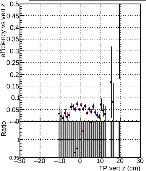
Efficiency vs vertpos Legend: DQM_TT_mkFit-DQM_original-0 DQM_TT_mkFit-DQM_mod-127 DQM_TT_mkFit-DQM_mod_updated-127
