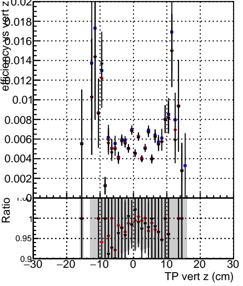
Efficiency vs vert z Legend: - DQM_TT_mkFit-DQM_original-0 (blue circles) - DQM_TT_mkFit-DQM_mod-127 (red circles) - DQM_TT_mkFit-DQM_updated-127 (black circles)
