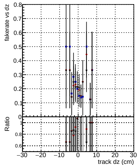
Fake rate vs dz Legend: DOM TT mkFit-DOM-original-0 DOM TT mkFit-DOM-mod-127 DOM TT mkFit-DOM-mod-updated-127
