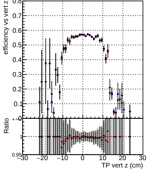
Efficiency vs vert z —●— DQM_TT_mkFit-DQM_original-0 —●— DQM_TT_mkFit-DQM_mod-127 —●— DQM_TT_mkFit-DQM_mod_updated-127
