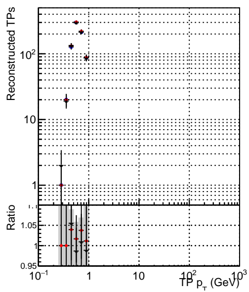
Legend: DQM_TT_mkFit-DQM_original-0 (blue dots), DQM_TT_mkFit-DQM_original-127 (red dots), DQM_TT_mkFit-DQM_updated-127 (black dots)
