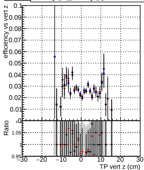
Efficiency vs. sim PV z — DQM_TT_mkFit-DQM_original-0 — DQM_TT_mkFit-DQM_original-127 — DQM_TT_mkFit-DQM_updated-127
