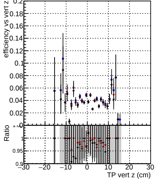
Efficiency vs vert z — DQM_TT_mkFit-DQM_original-0 — DQM_TT_mkFit-DQM_original-127 — DQM_TT_mkFit-DQM_updated-127
